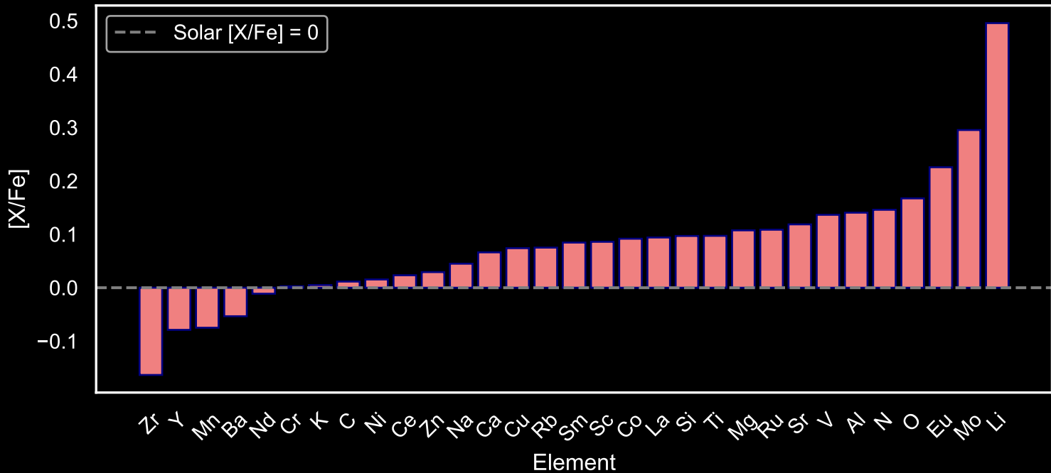
Abundance Pattern for GALAH Star Field [26] (N=289)
