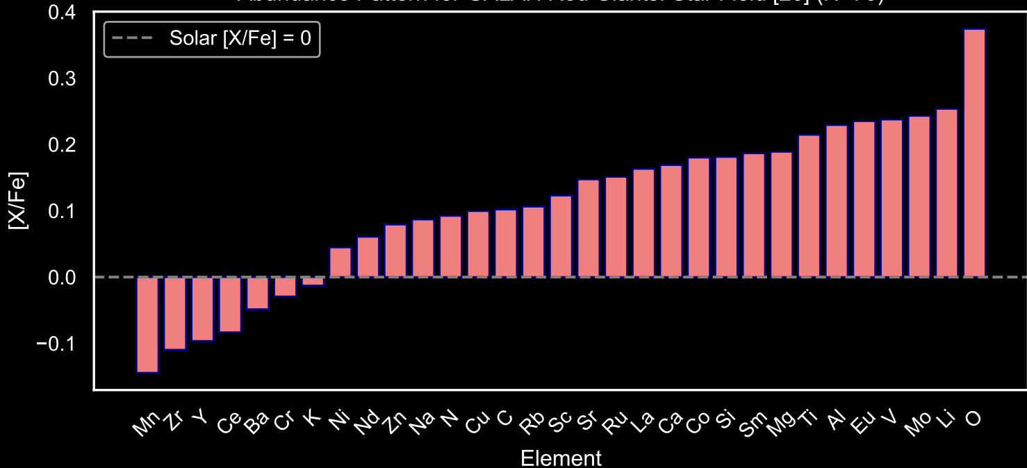
Abundance Pattern for GALAH Red Giants: Star Field [26] (N=70)
