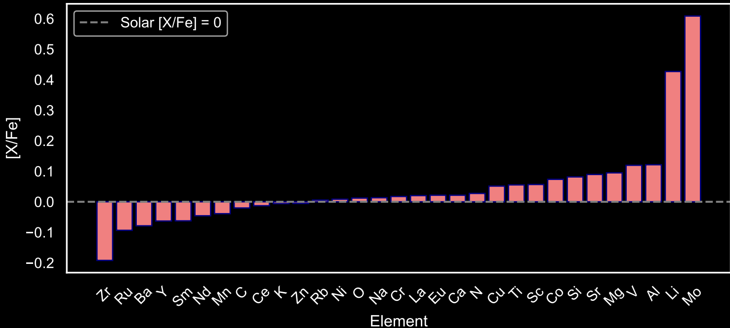
Abundance Pattern for GALAH Main Sequence Stars: Star Field [26] (N=126)
